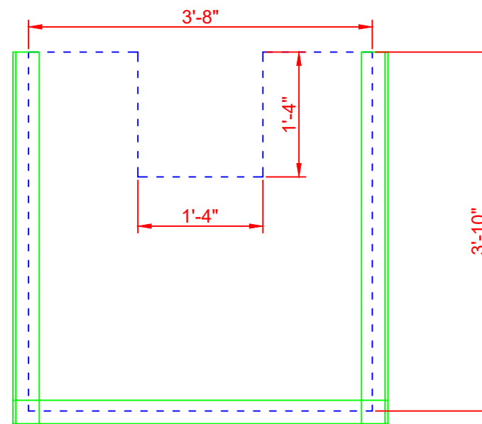
WEIR PLATE
