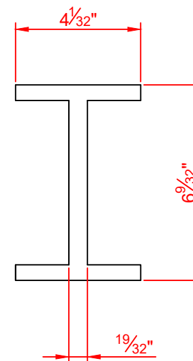
6" Wide flange (6WF#16)
