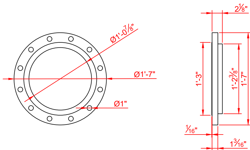
Slip On RF 12" Flange x 150 Class 12 holes x 1" diameter
