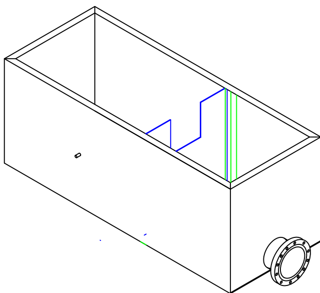
WEIR BOX ISOMETRIC VIEW
